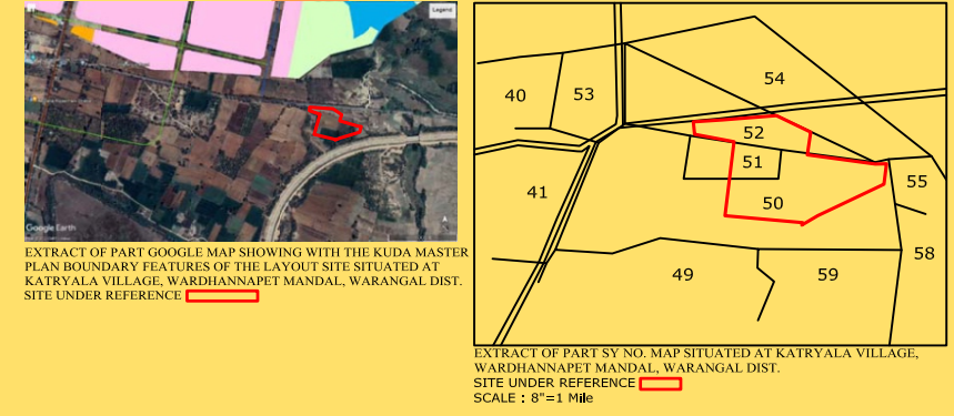
EXTRACT OF PART SY NO. MAP SITUATED AT KATRYALA VILLAGE, WARDHANNAPET MANDAL, WARANGAL DIST.
